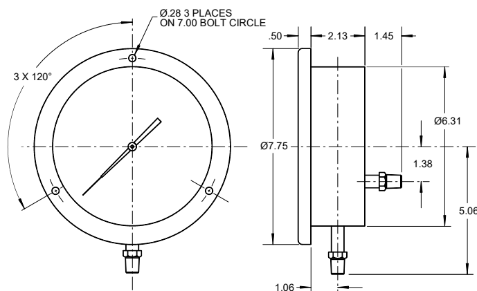
6" Front Flange
