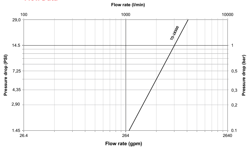
Air flow-rate at 6 bar (87 psi)
