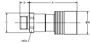
Figure 3 Male ORB
