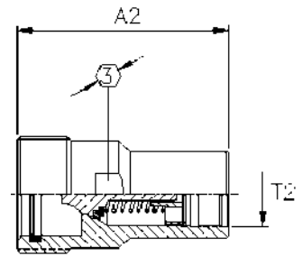
Female Half
