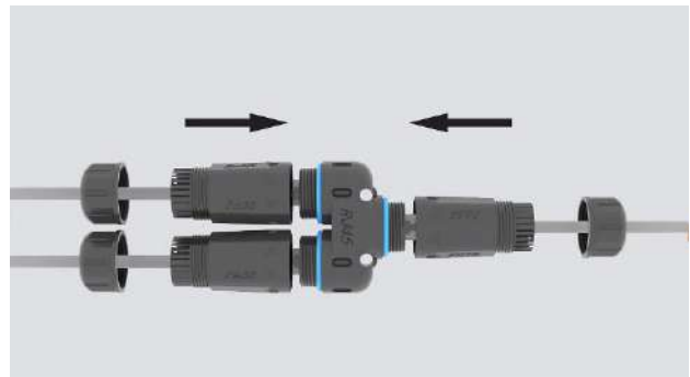
IP68 SPLITTER
