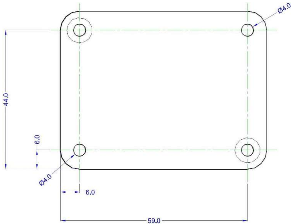
Figure 1 Mounting Drawing
