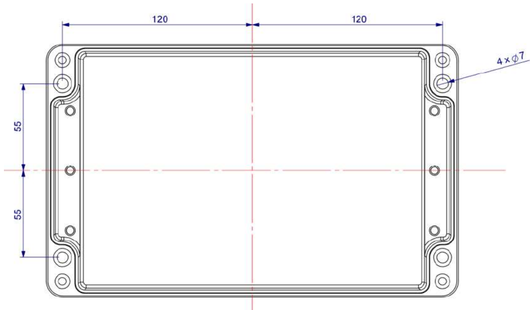
Operator Console Dimensions
