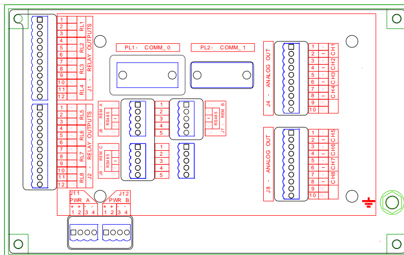
Operator Console – Rear Panel Connectors
