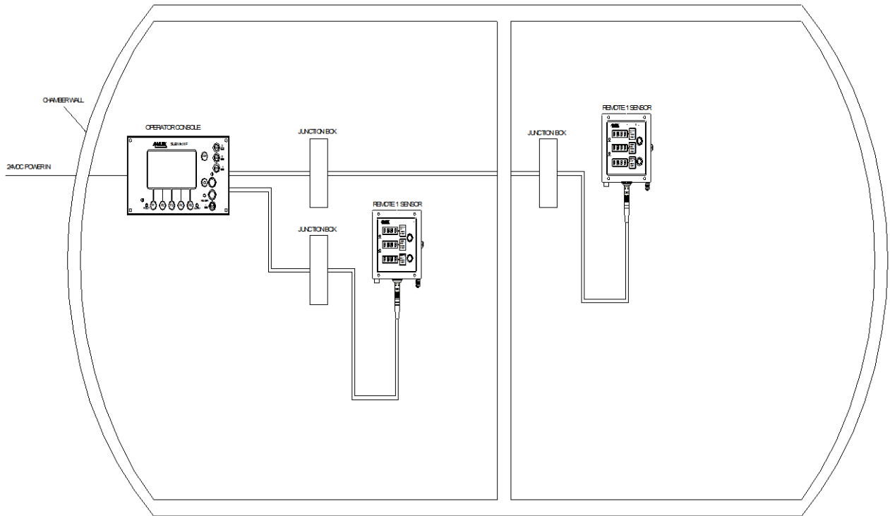
Figure 2 Typical Monitoring System in a Submarine Rescue Vehicle (2 compartments)
