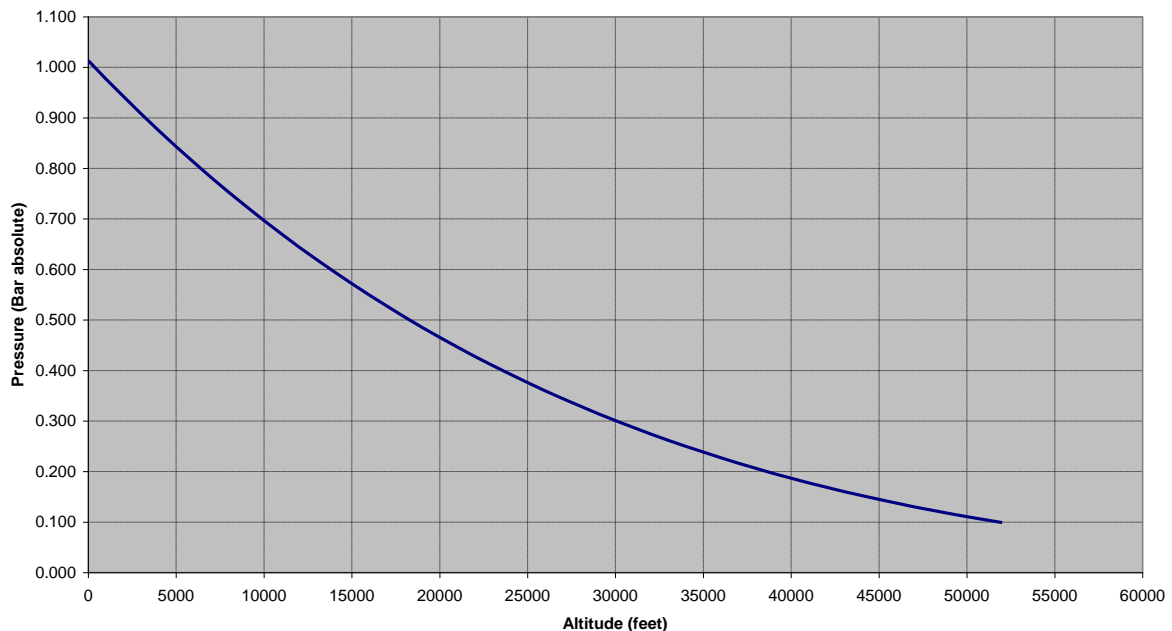
Pressure/Altitude Conversion
