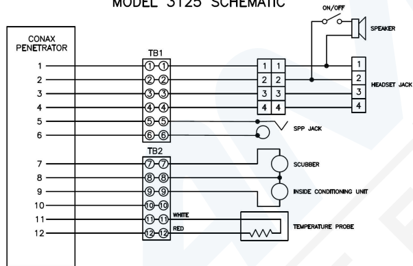
MODEL 3125 SCHEMATIC
