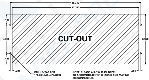
FIGURE 1 - RACK MOUNT COMMUNICATOR MOUNTING DIMENSIONS
